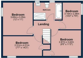
First Floor Approx. 52.8 sq. metres (568.1 sq. feet)
